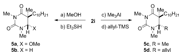
Scheme 2. Reactivity of the tetrahedral adducts 2 . Reaction conditions: a) MeOH, HCl, RT, 3 h, 99%. b) Et 3 SiH, BF 3 ·Et 2 O, RT, 3 h, 96%. c) Me 3 Al, RT, 3 h, 78%. d) allyl-TMS, BF 3 ·Et 2 O, RT, 2 h, 86%.
